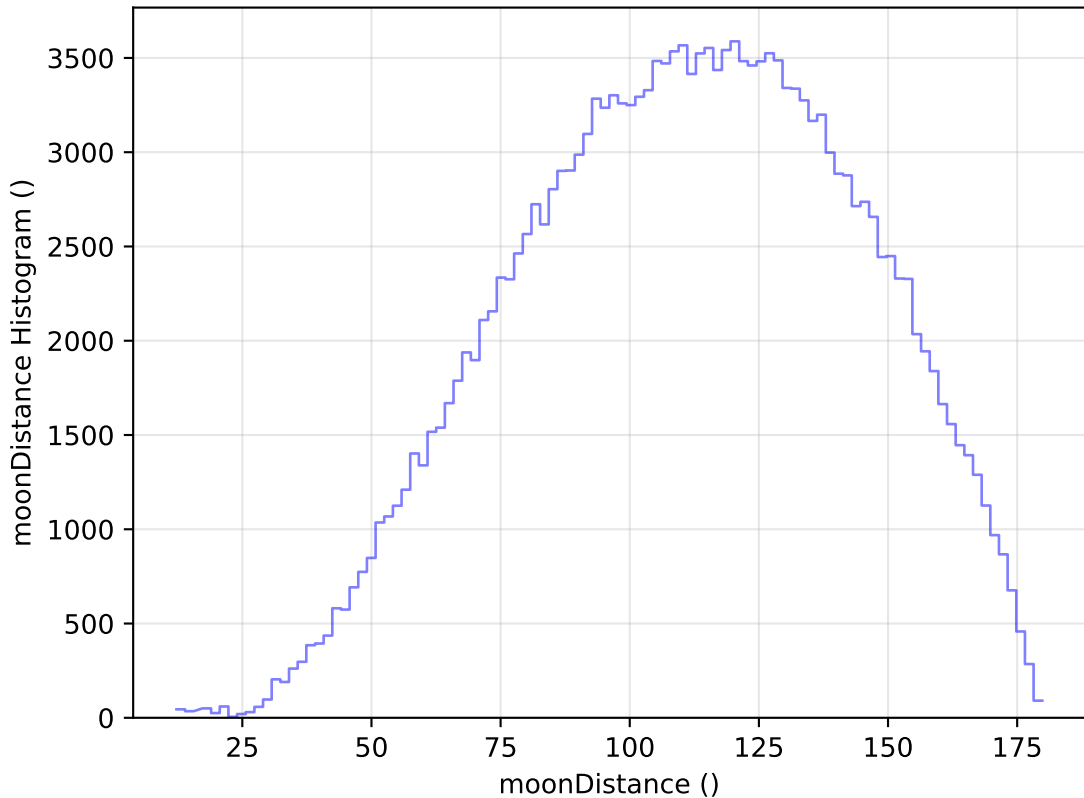
ddf_loaded_half_fl15_v3.4_10yrs All sky g band: moonDistance Histogram
