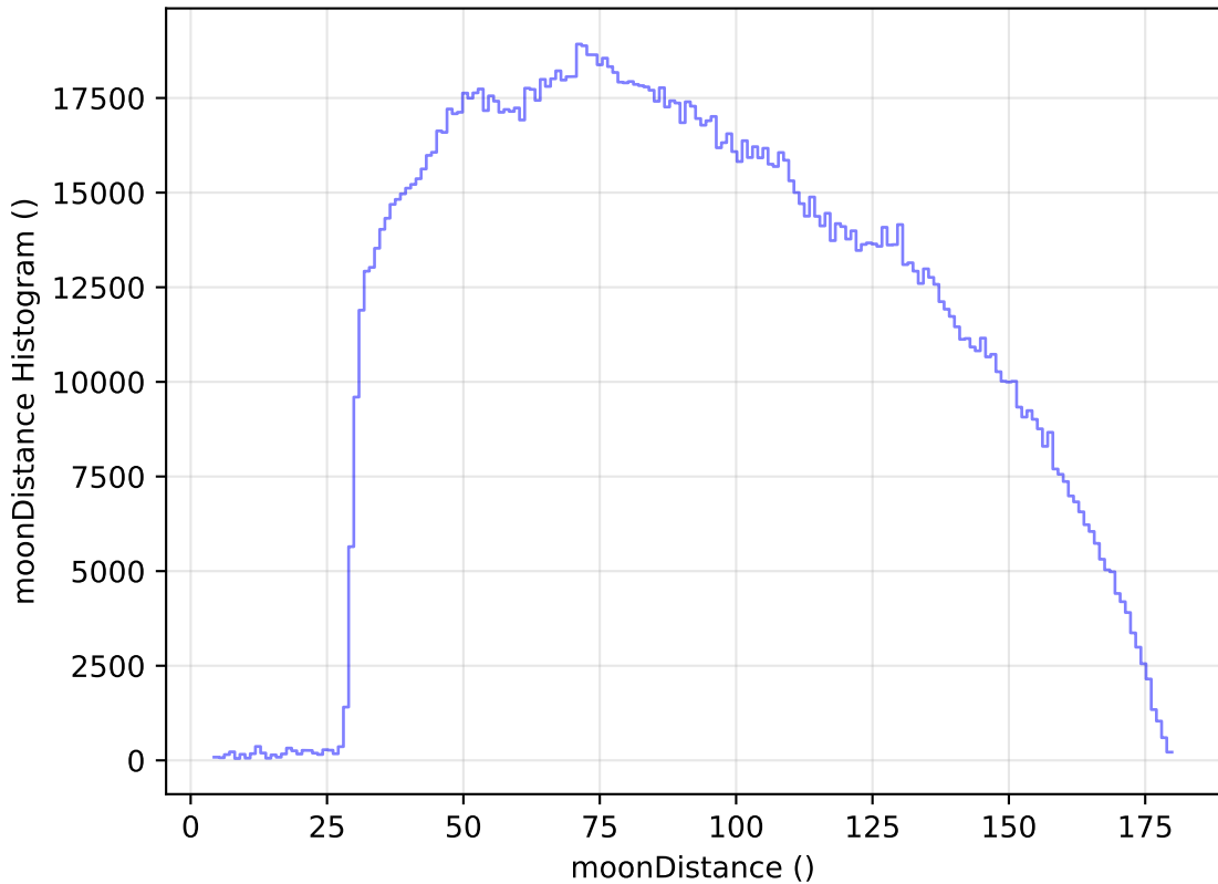
ddf_loaded_half_fl15_v3.4_10yrs All sky all bands: moonDistance Histogram
