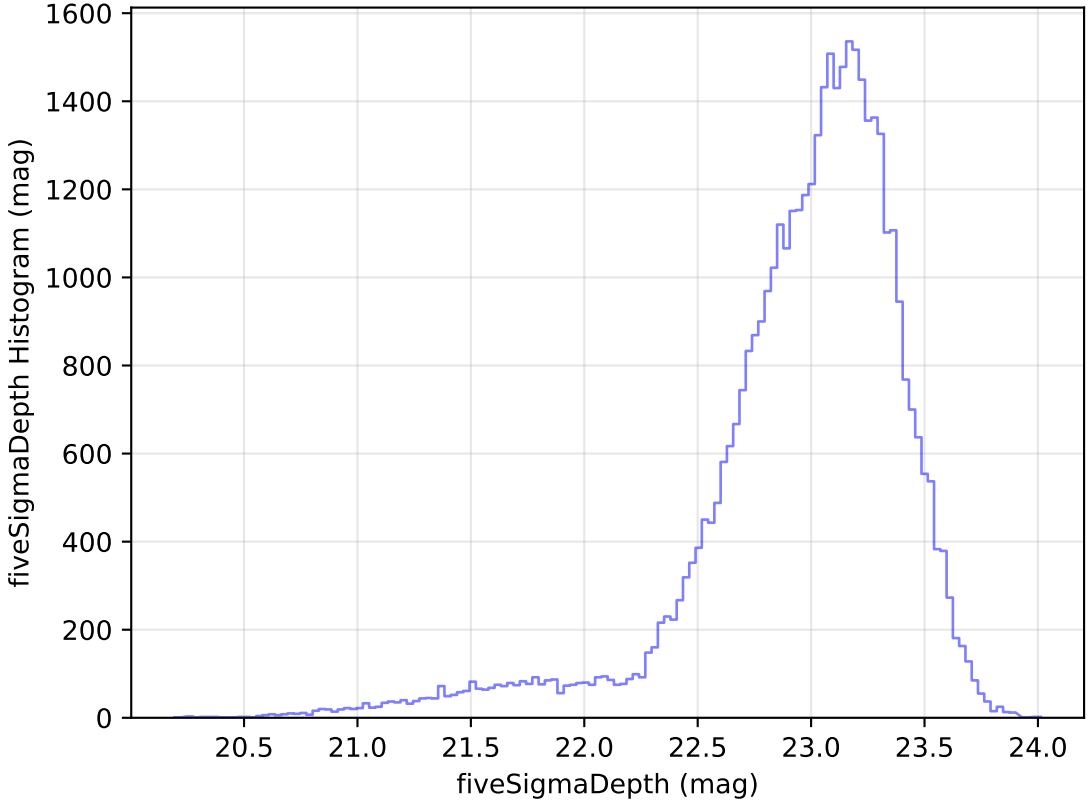
ddf_loaded_half_fl15_v3.4_10yrs Yr 1 z band: fiveSigmaDepth Histogram
