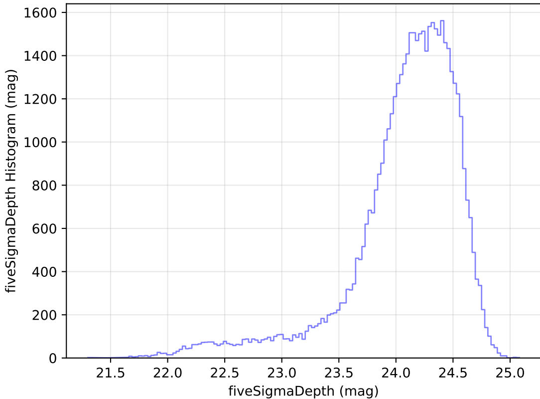
ddf_loaded_half_fl15_v3.4_10yrs Yr 1 r band: fiveSigmaDepth Histogram
