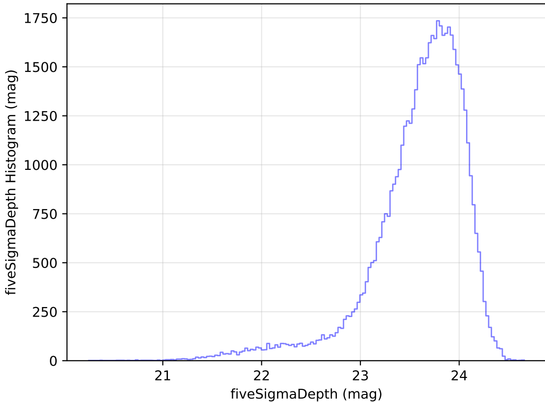
ddf_loaded_half_fl15_v3.4_10yrs Yr 1 i band: fiveSigmaDepth Histogram
