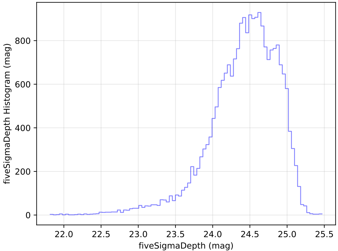
ddf_loaded_half_fl15_v3.4_10yrs Yr 1 g band: fiveSigmaDepth Histogram
