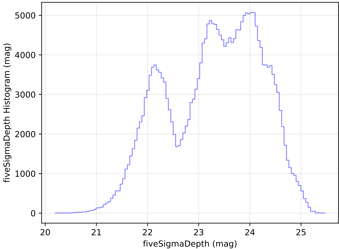
ddf_loaded_half_fl15_v3.4_10yrs Yr 1 all bands: fiveSigmaDepth Histogram
