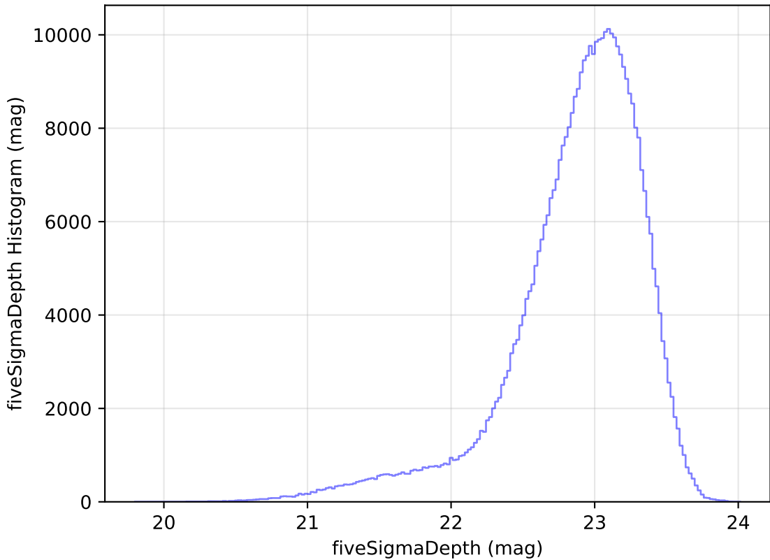
ddf_loaded_half_fl15_v3.4_10yrs WFD z band: fiveSigmaDepth Histogram
