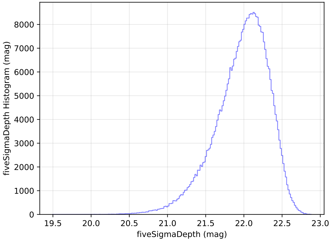
ddf_loaded_half_fl15_v3.4_10yrs WFD y band: fiveSigmaDepth Histogram
