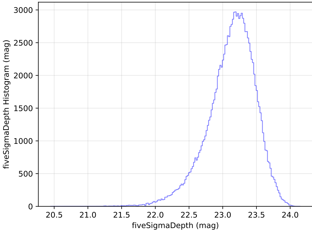
ddf_loaded_half_fl15_v3.4_10yrs WFD u band: fiveSigmaDepth Histogram
