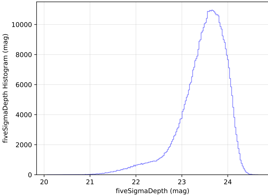
ddf_loaded_half_fl15_v3.4_10yrs WFD i band: fiveSigmaDepth Histogram
