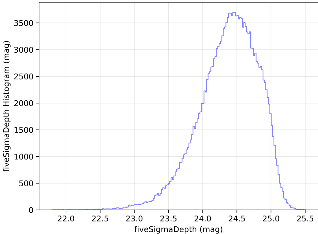
ddf_loaded_half_fl15_v3.4_10yrs WFD g band: fiveSigmaDepth Histogram
