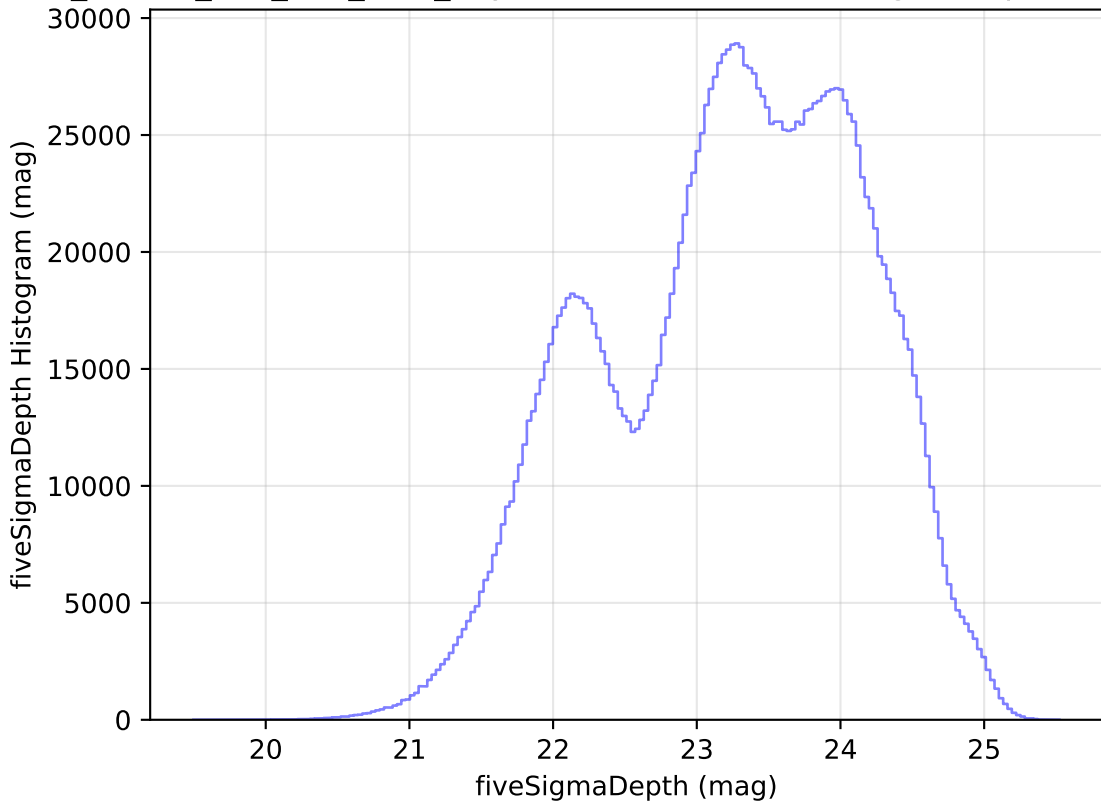
ddf_loaded_half_fl15_v3.4_10yrs WFD all bands: fiveSigmaDepth Histogram
