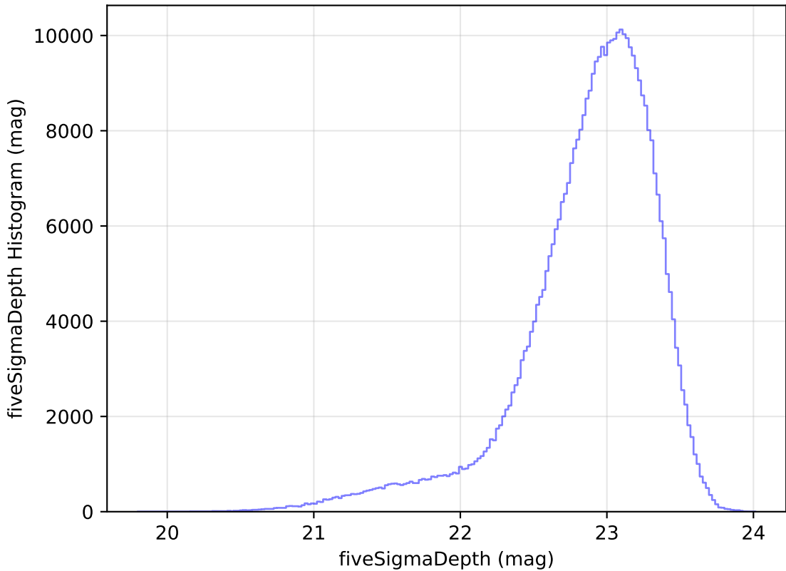
ddf_loaded_half_fl15_v3.4_10yrs All sky z band: fiveSigmaDepth Histogram
