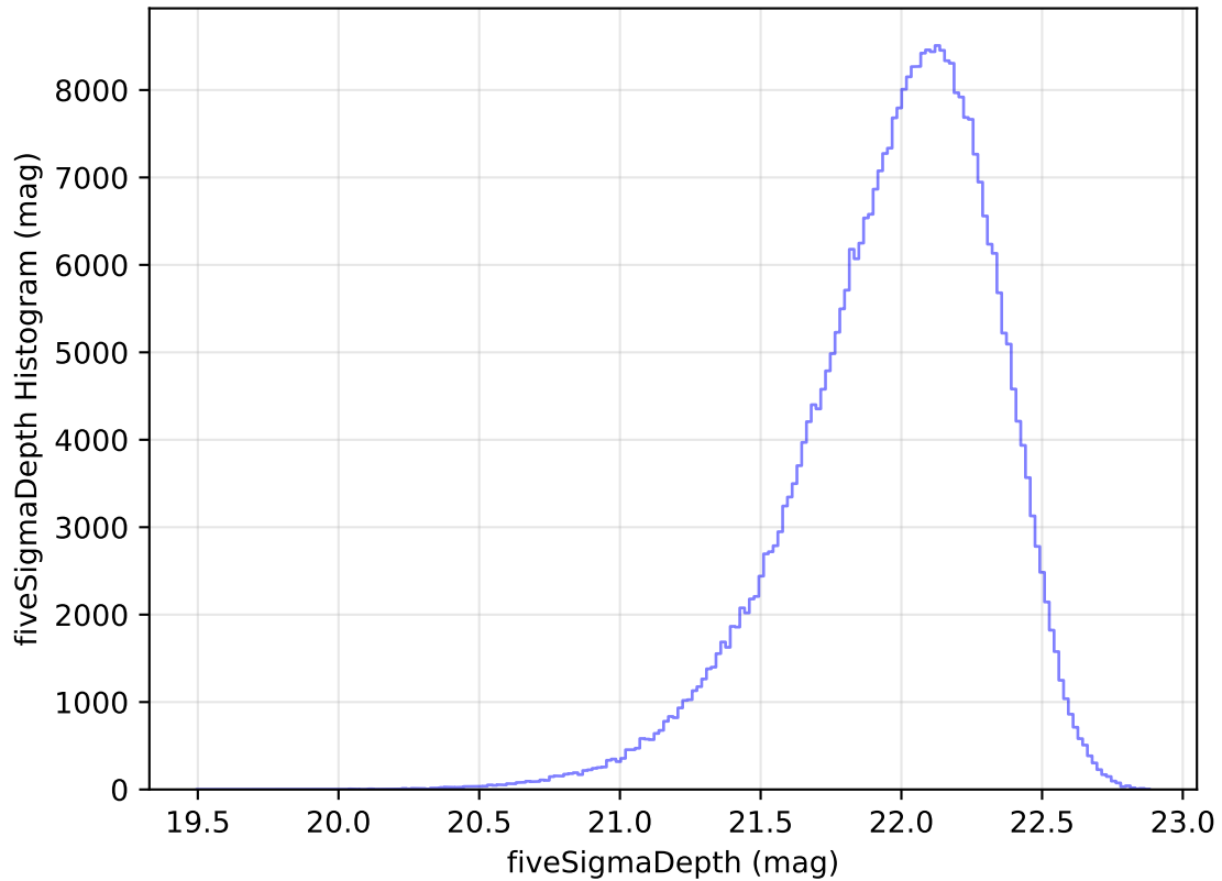
ddf_loaded_half_fl15_v3.4_10yrs All sky y band: fiveSigmaDepth Histogram
