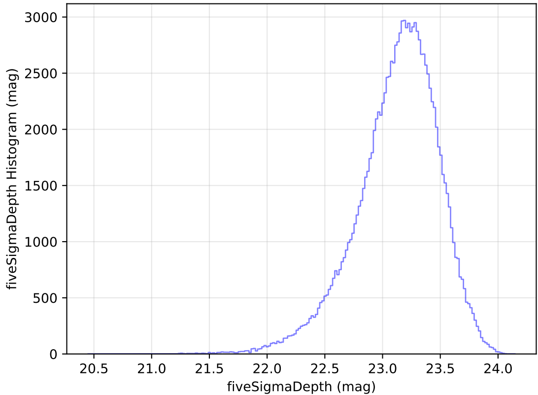
ddf_loaded_half_fl15_v3.4_10yrs All sky u band: fiveSigmaDepth Histogram
