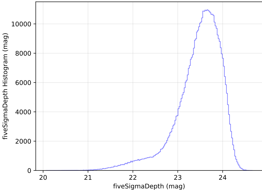
ddf_loaded_half_fl15_v3.4_10yrs All sky i band: fiveSigmaDepth Histogram
