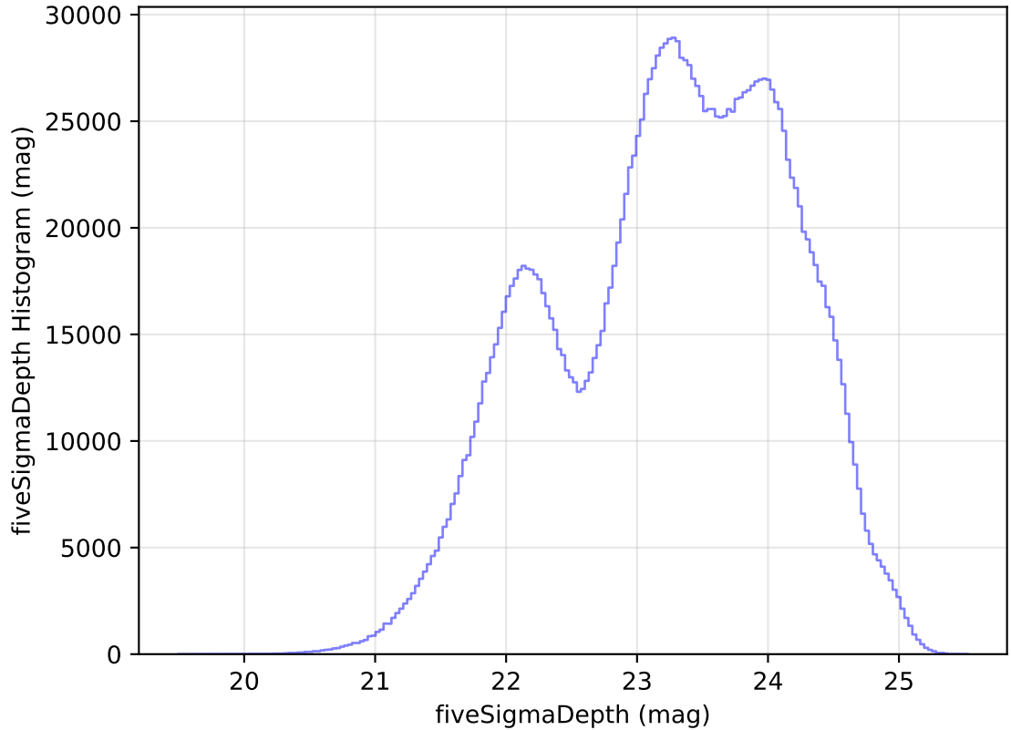
ddf_loaded_half_fl15_v3.4_10yrs All sky all bands: fiveSigmaDepth Histogram
