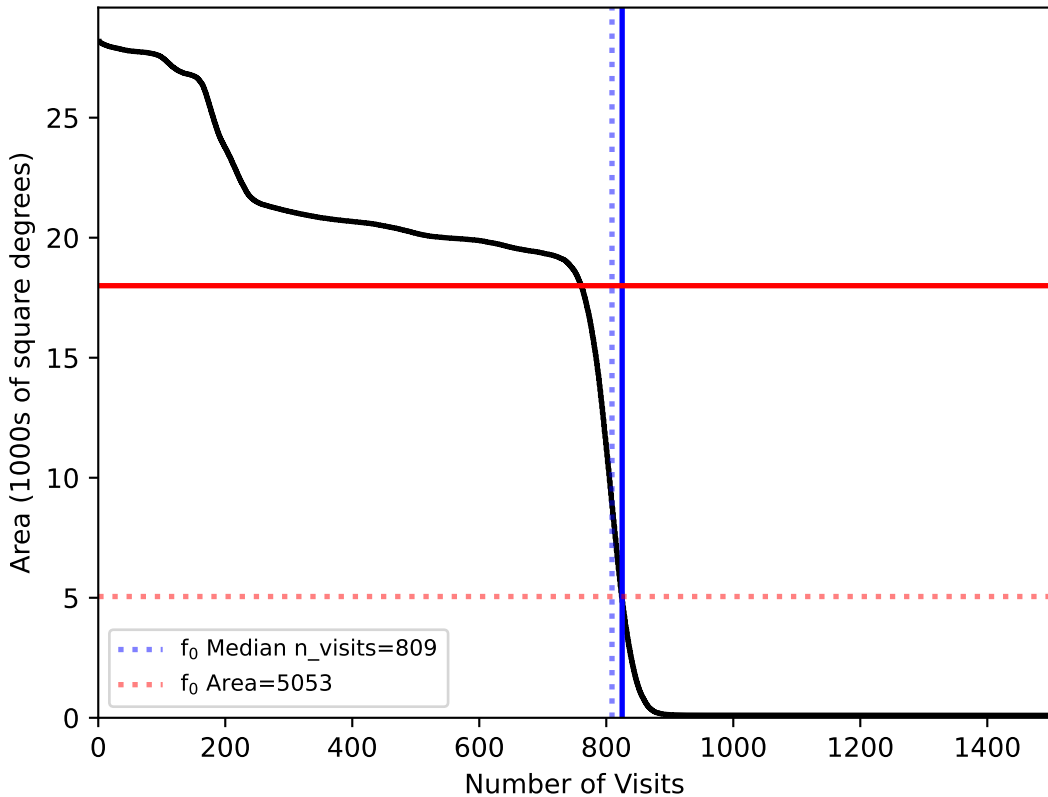
ddf_loaded_half_fl15_v3.4_10yrs All sky: f0
