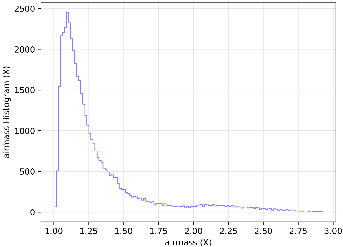
ddf_loaded_half_fl15_v3.4_10yrs Yr 1 z band: airmass Histogram
