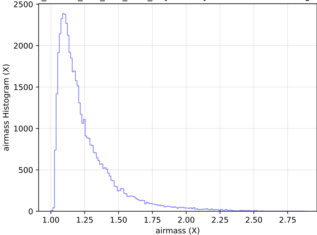
ddf_loaded_half_fl15_v3.4_10yrs Yr 1 y band: airmass Histogram
