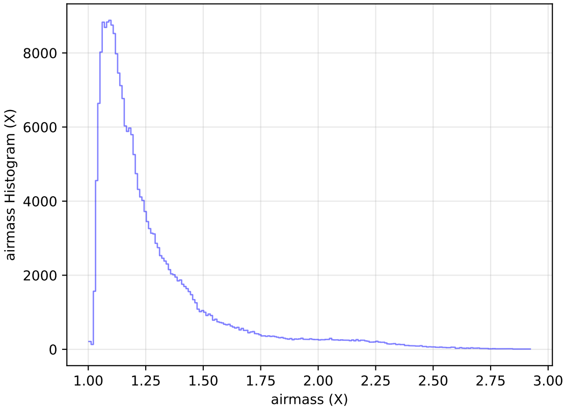
ddf_loaded_half_fl15_v3.4_10yrs Yr 1 all bands: airmass Histogram
