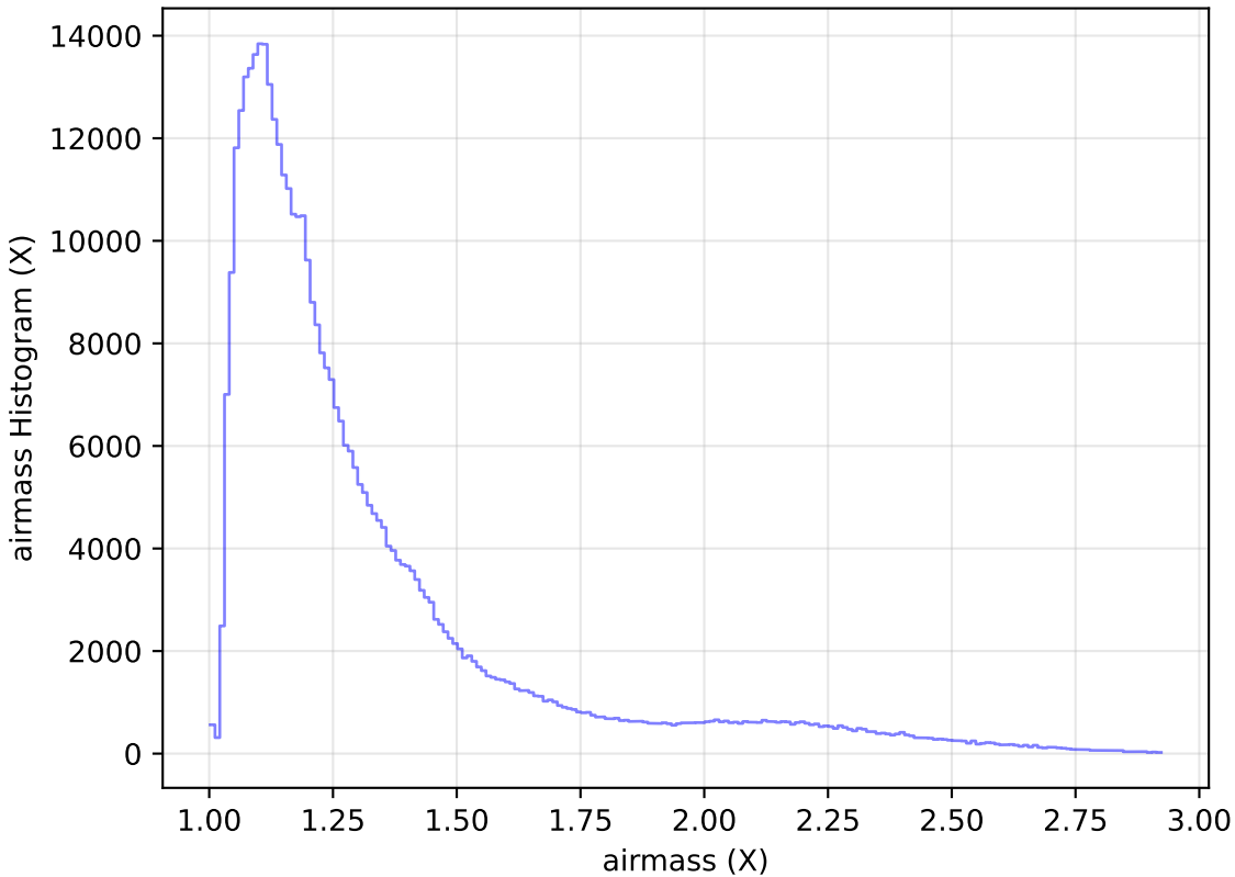
ddf_loaded_half_fl15_v3.4_10yrs WFD z band: airmass Histogram
