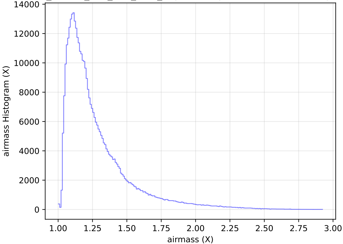
ddf_loaded_half_fl15_v3.4_10yrs WFD y band: airmass Histogram
