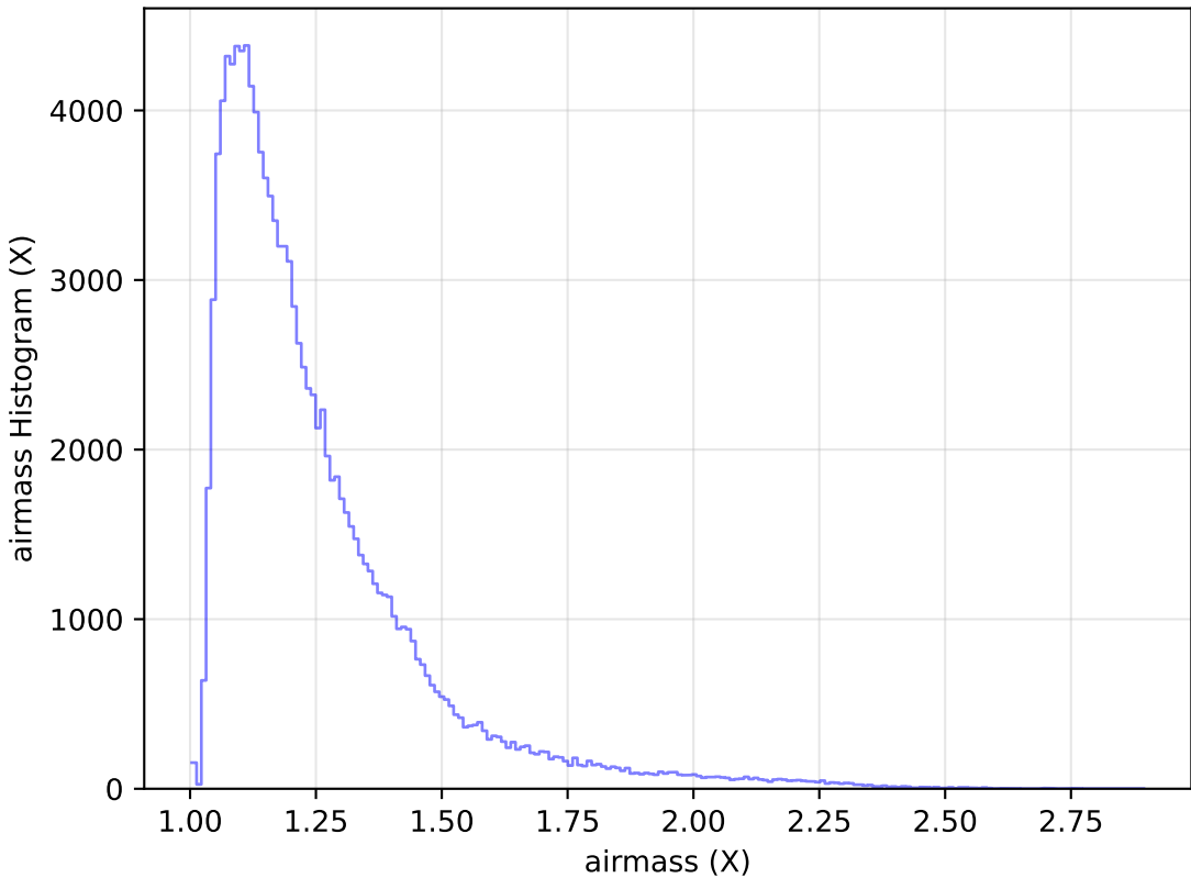
ddf_loaded_half_fl15_v3.4_10yrs WFD u band: airmass Histogram
