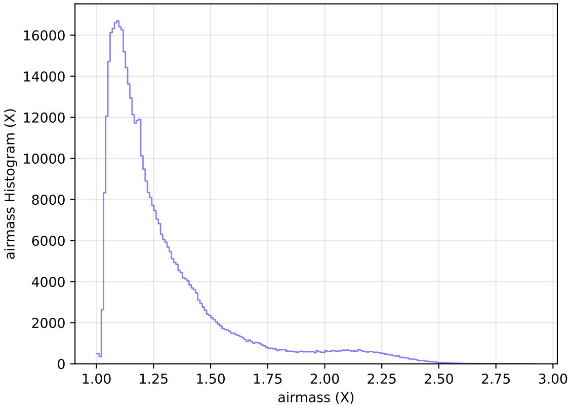
ddf_loaded_half_fl15_v3.4_10yrs WFD r band: airmass Histogram
