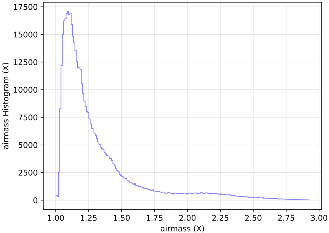
ddf_loaded_half_fl15_v3.4_10yrs WFD i band: airmass Histogram
