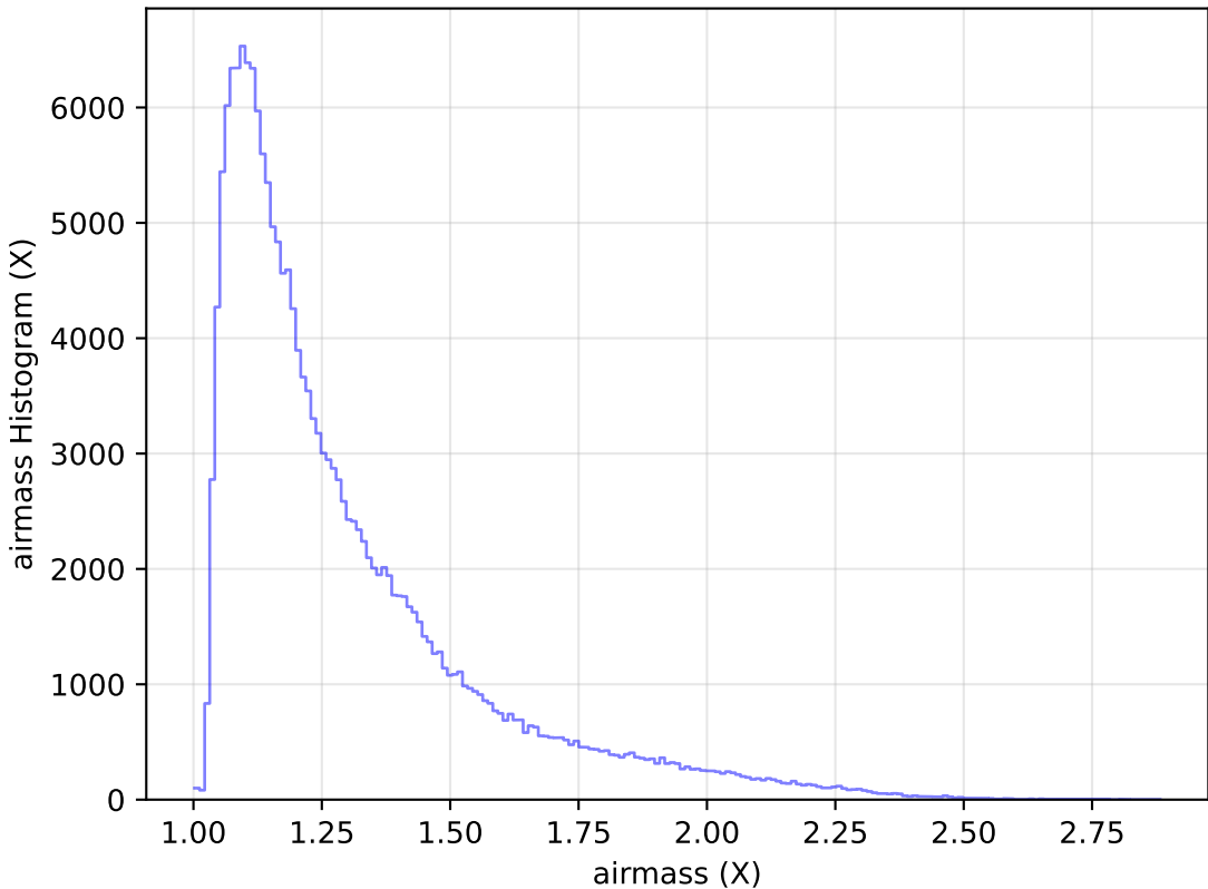
ddf_loaded_half_fl15_v3.4_10yrs WFD g band: airmass Histogram
