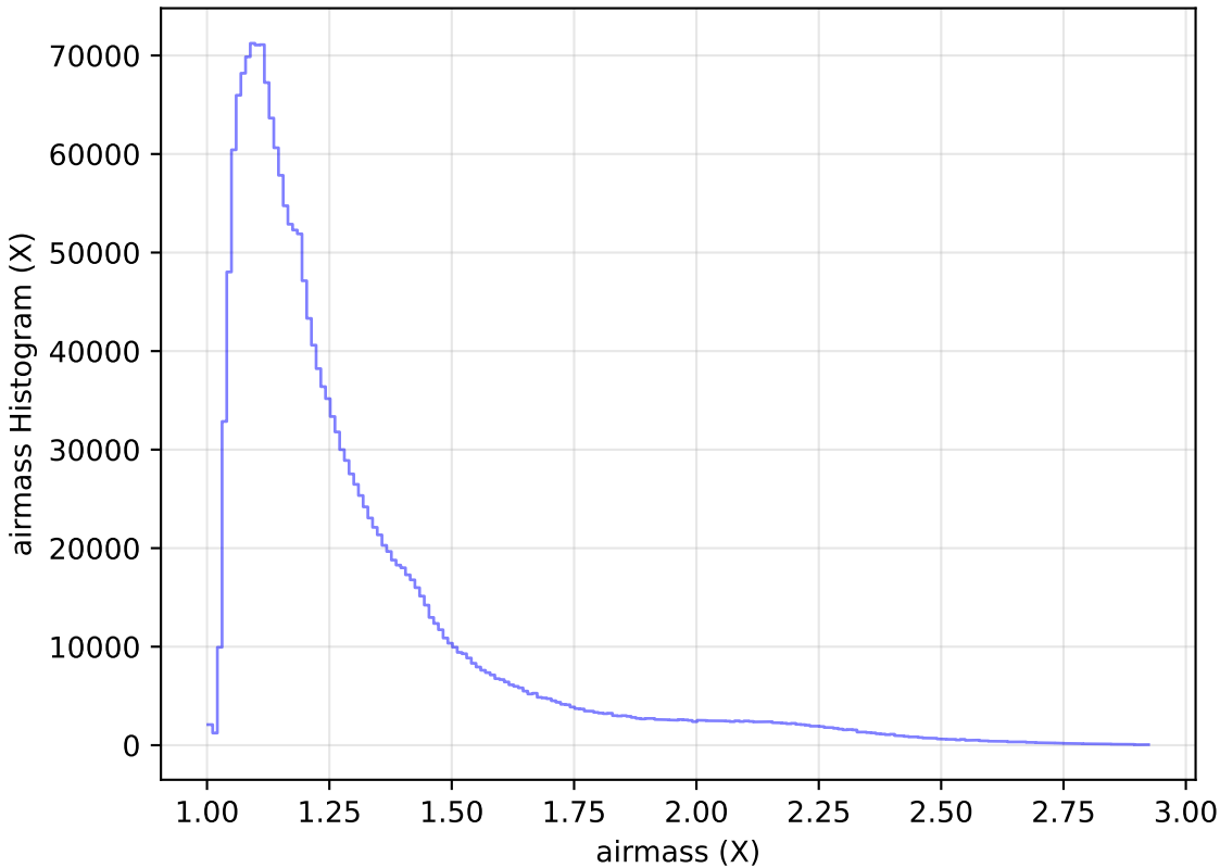
ddf_loaded_half_fl15_v3.4_10yrs WFD all bands: airmass Histogram
