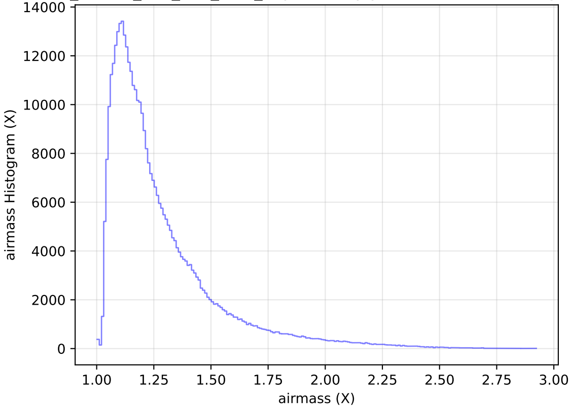
ddf_loaded_half_fl15_v3.4_10yrs All sky y band: airmass Histogram
