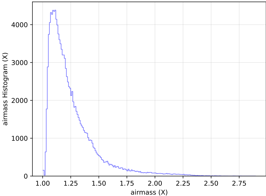
ddf_loaded_half_fl15_v3.4_10yrs All sky u band: airmass Histogram
