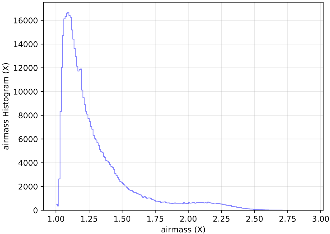
ddf_loaded_half_fl15_v3.4_10yrs All sky r band: airmass Histogram
