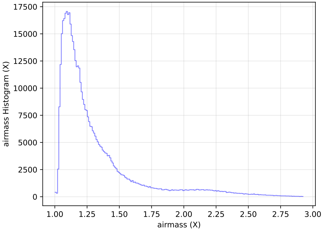
ddf_loaded_half_fl15_v3.4_10yrs All sky i band: airmass Histogram
