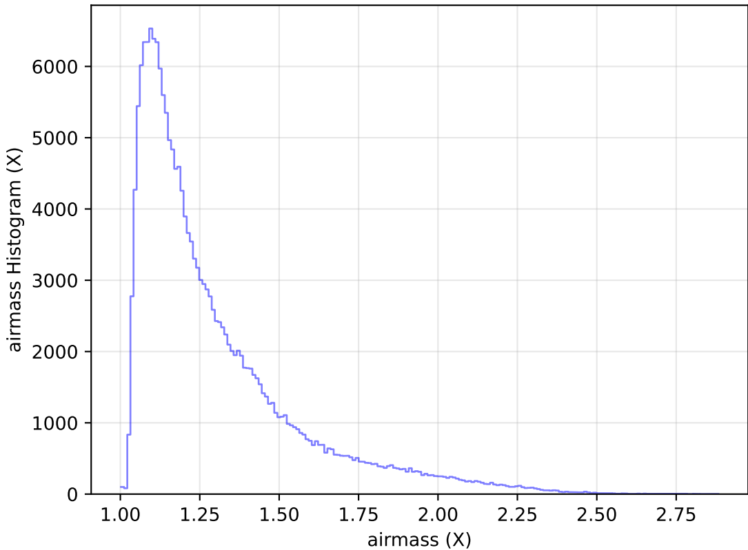
ddf_loaded_half_fl15_v3.4_10yrs All sky g band: airmass Histogram
