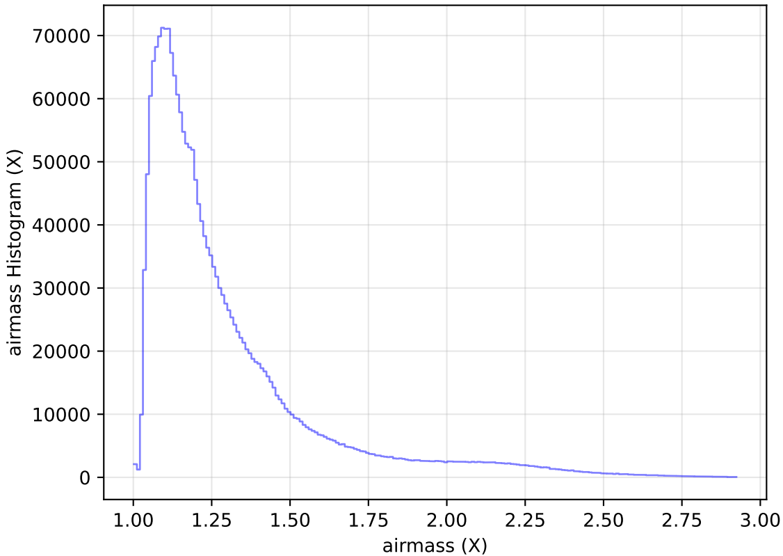
ddf_loaded_half_fl15_v3.4_10yrs All sky all bands: airmass Histogram
