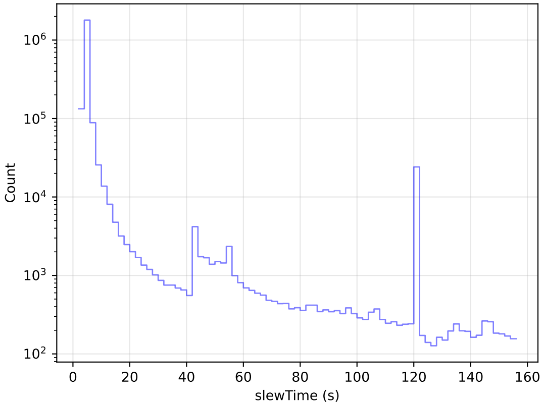
ddf_loaded_half_fl15_v3.4_10yrs All visits: Slew Time Histogram
