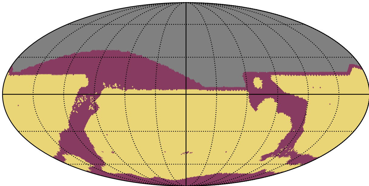
ddf_loaded_half_fl15_v3.4_10yrs All sky: RapidRevisits
