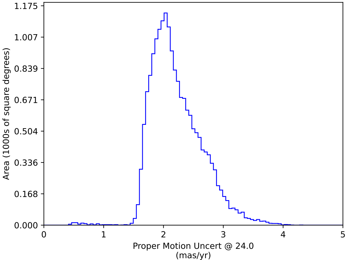
ddf_loaded_half_fl15_v3.4_10yrs WFD: Proper Motion Uncert @ 24.0
