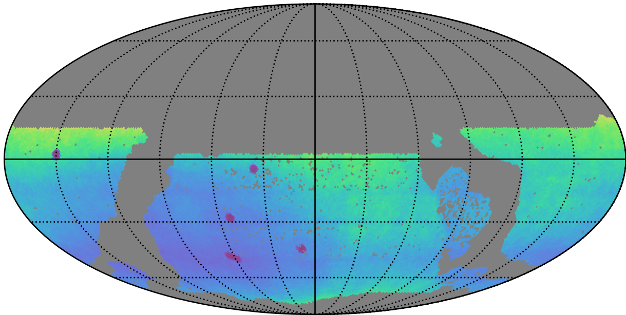
ddf_loaded_half_fl15_v3.4_10yrs WFD: Parallax Uncert @ 24.0
