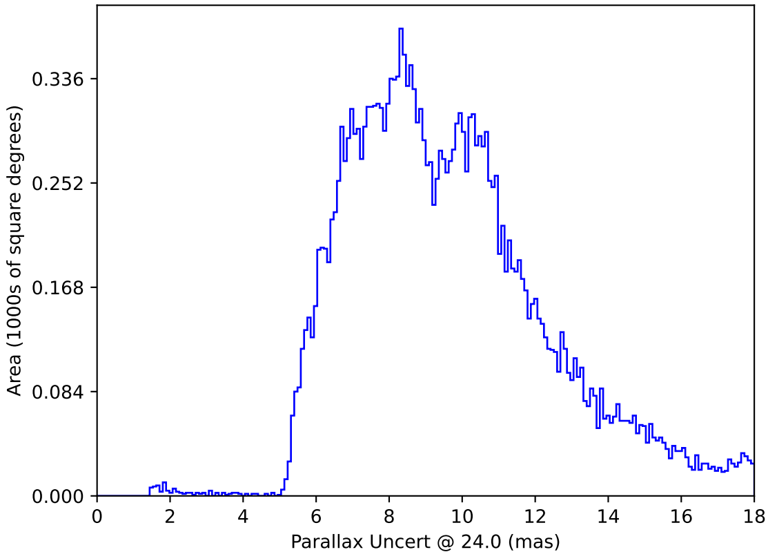
ddf_loaded_half_fl15_v3.4_10yrs All sky: Parallax Uncert @ 24.0
