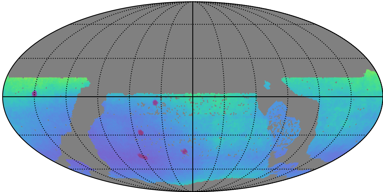
ddf_loaded_half_fl15_v3.4_10yrs WFD: Parallax Uncert @ 22.4
