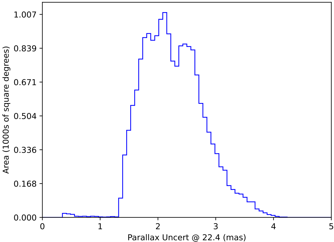
ddf_loaded_half_fl15_v3.4_10yrs WFD: Parallax Uncert @ 22.4
