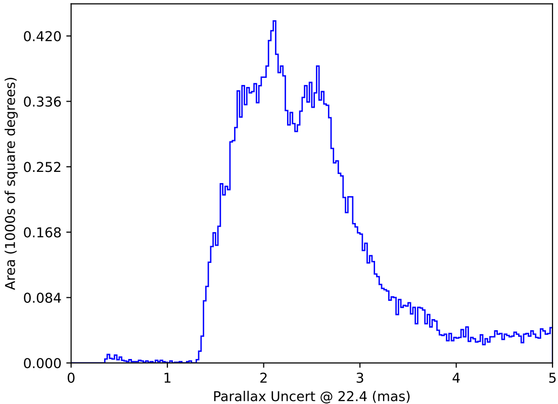
ddf_loaded_half_fl15_v3.4_10yrs All sky: Parallax Uncert @ 22.4
