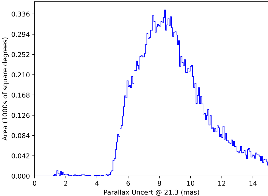
ddf_loaded_half_fl15_v3.4_10yrs All sky y band only: Parallax Uncert @ 21.3
