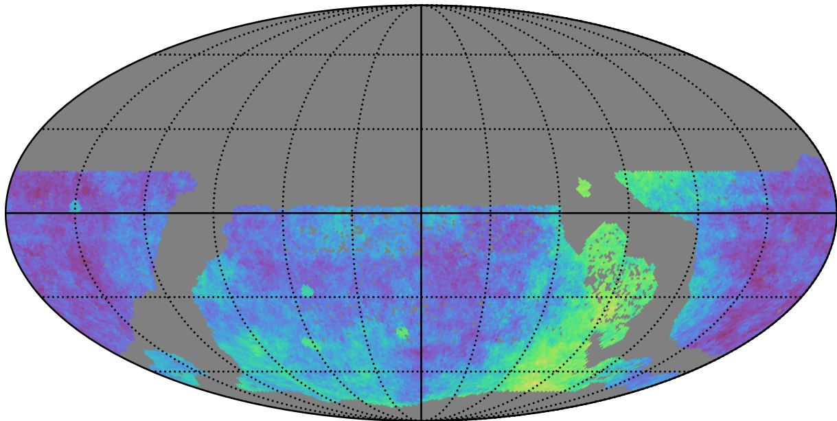
ddf_loaded_half_fl15_v3.4_10yrs WFD: Parallax Coverage @ 24.0
