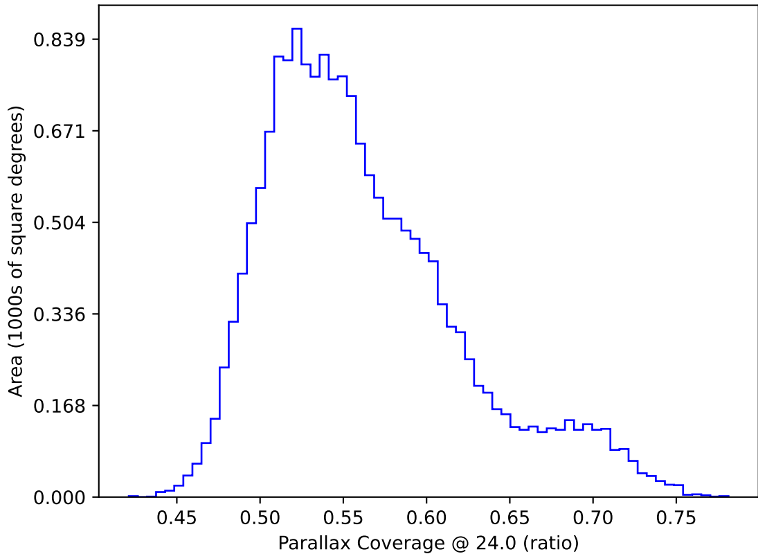
ddf_loaded_half_fl15_v3.4_10yrs WFD: Parallax Coverage @ 24.0
