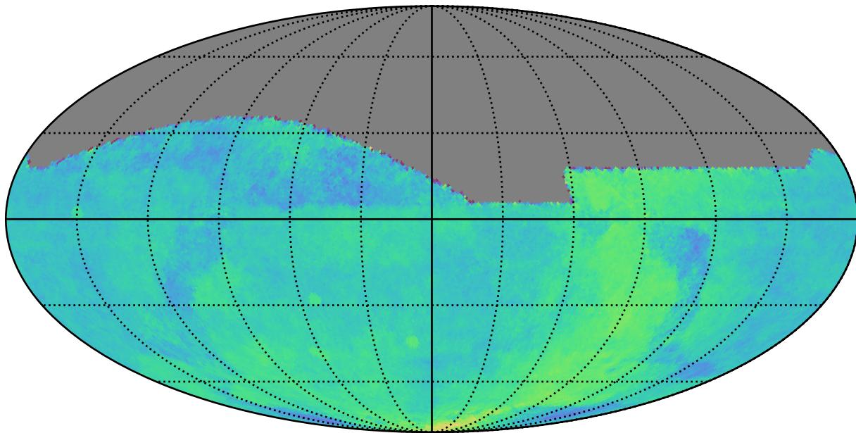
ddf_loaded_half_fl15_v3.4_10yrs All sky: Parallax Coverage @ 24.0
