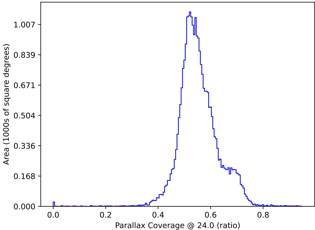
ddf_loaded_half_fl15_v3.4_10yrs All sky: Parallax Coverage @ 24.0
