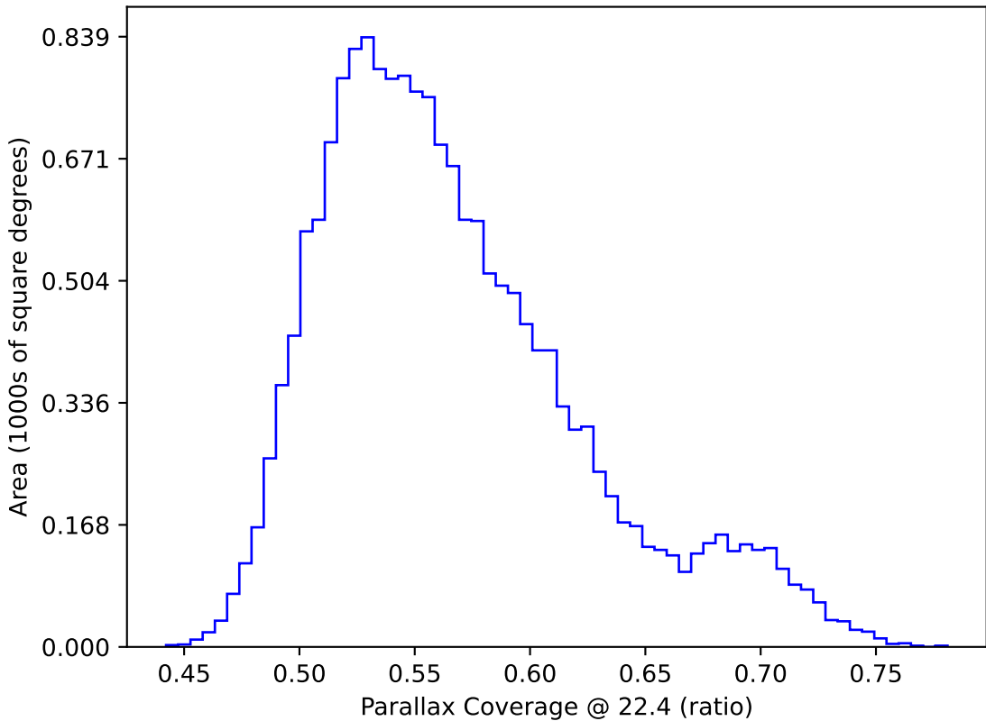
ddf_loaded_half_fl15_v3.4_10yrs WFD: Parallax Coverage @ 22.4
