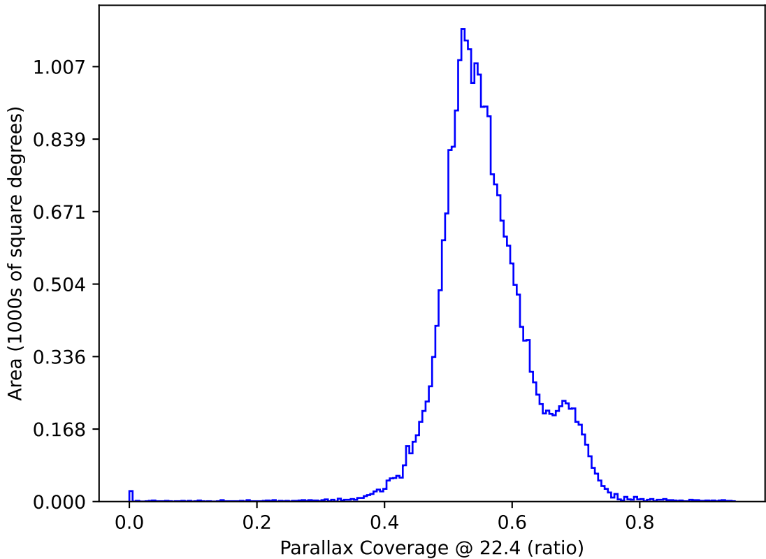
ddf_loaded_half_fl15_v3.4_10yrs All sky: Parallax Coverage @ 22.4
